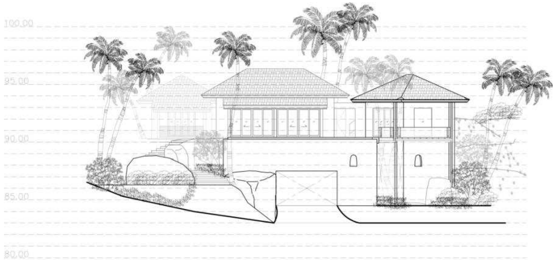
FRONT ELEVATION VILLA : PLOT 1
